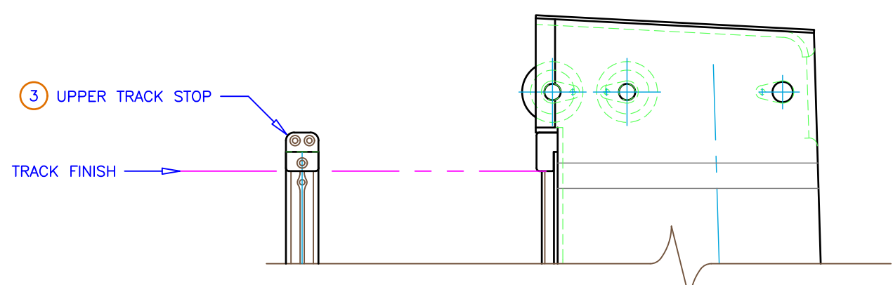
UPPER AND LOWER DETAIL SCALE: 1:5
